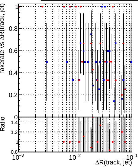
Fake rate vs \Delta R(\text{track, jet}) Legend: \blacksquare DQM_CKF_XiMinusNOPU_base \bullet DQM_CKF_XiMinusNOPU_retrainOldFiles125_v2_prelimWPM_epoch1
