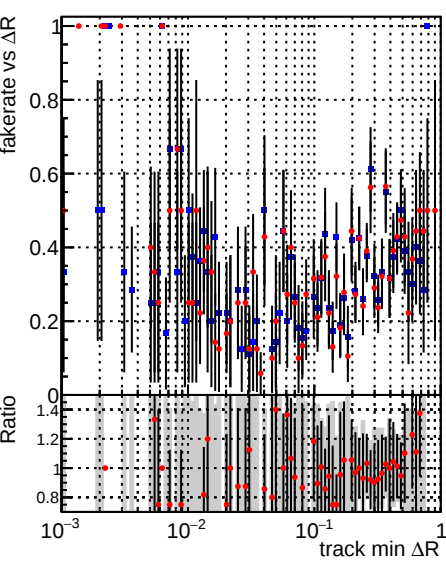
Fake rate vs \Delta R(\text{track, jet}) Legend: \blacksquare DQM_CKF_XiMinusNOPU_base \bullet DQM_CKF_XiMinusNOPU_retrainOldFiles125_v2_prelimWPM_epoch1
