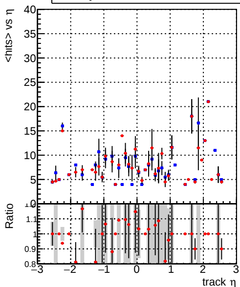
mean hits vs \eta — DQM_CKF_XiMinusNOPU_base — DQM_CKF_XiMinusNOPU_retrainOldFiles125_v2_prelimWPM_epoch1
