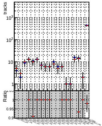
N of reco track vs. \chi^2 —●— DQM_CKF_XiMinusNOPU_base —●— DQM_CKF_XiMinusNOPU_retrainOldFiles125_v2_prelimWPM_epoch1
