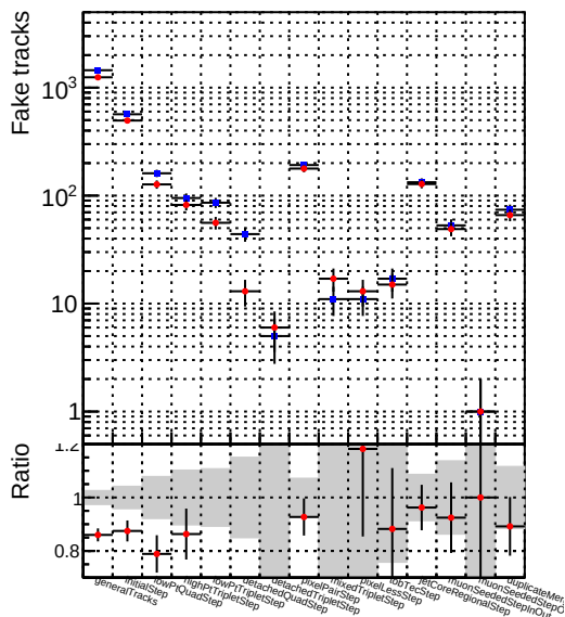
Number —●— DQM_CKF_XiMinusNOPU_retrainOldFiles125_v2_prelimWPM_epoch1
