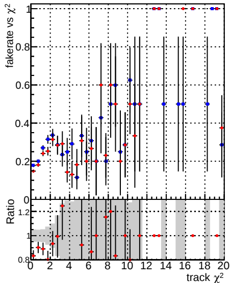
Fake rate vs. \chi^2 —●— DQM_CKF_XiMinusNOPU_base —●— DQM_CKF_XiMinusNOPU_retrainOldFiles125_v2_prelimWPM_epoch1
