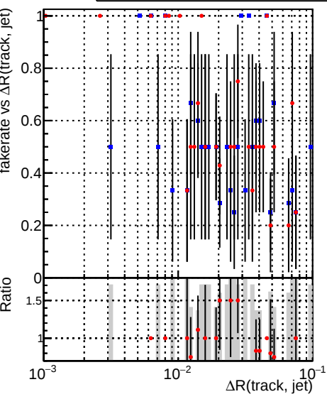
Legend: \blacksquare DQM_CKF_XiMinusNOPU_base \bullet DQM_CKF_XiMinusNOPU_retrainOldFiles125_v2_prelimWPM_epoch1
