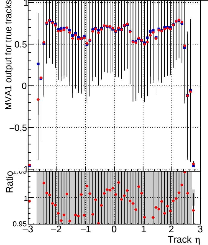
MVA1 of associated tracks (recoToSim) vs. track \eta Legend: ■ DQM_CKF_XiMinusNOPU_base ● DQM_CKF_XiMinusNOPU_retrainOldFiles125_v2_prelimWPM_epoch1
