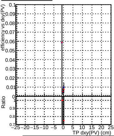
Efficiency vs Dxy(PV) Legend: DQM_CKF_XiMinusNOPU_base (blue square), DQM_CKF_XiMinusNOPU_retrainOldFiles125_v2_prelimWPM_epoch1 (red circle)
