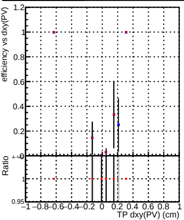
Efficiency vs Dxy(PV) Legend: DQM_CKF_XiMinusNOPU_base (blue square), DQM_CKF_XiMinusNOPU_retrainOldFiles125_v2_prelimWPM_epoch1 (red circle)
