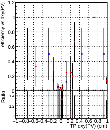
Efficiency vs Dxy(PV) - DQM_CKF_XiMinusNOPU_base - DQM_CKF_XiMinusNOPU_retrainOldFiles125_v2_prelimWPM_epoch1
