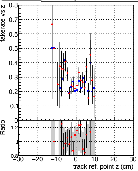
Legend: DQM_CKF_XiMinusNOPU_base (blue squares), DQM_CKF_XiMinusNOPU_retrainOldFiles125_v2_prelimWPM_epoch1 (red circles)
