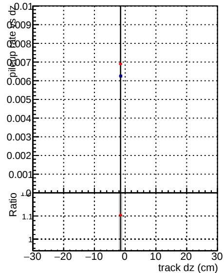
DQM_CKF_XiMinusNOPU_retrainOldFiles125_v2_prelimWPM_epoch1
