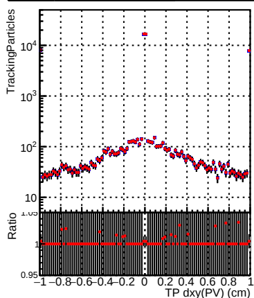
N of sim —●— DQM_CKF_XiMinusNO
