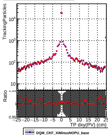
N of sim —●— DQM_CKF_XiMinusNO
