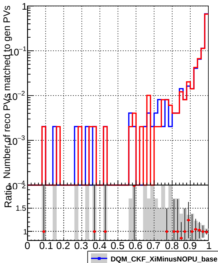
RecoPVAssoc2GenPVMatched_Purity
