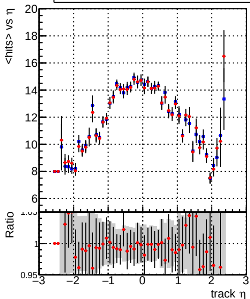
mean hit — DQM_CKF_XiMinusNOPU_base — DQM_CKF_XiMinusNOPU_retrainOldFiles125_v2_prelimWPM_epoch0
