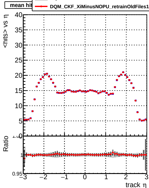
mean hits vs \eta
