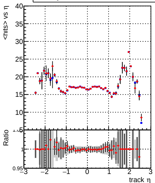
mean hits vs \eta Legend: DQM_CKF_XiMinusNOPU_base (blue line), DQM_CKF_XiMinusNOPU_retrainOldFiles125_v2_prelimWPM_epoch0 (red line)
