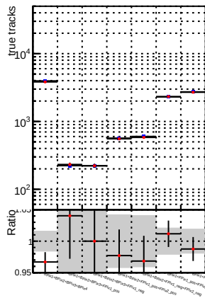
N of reco track vs. \chi^2 DOM_CKF_XiMinusNOPU_base DOM_CKF_XiMinusNOPU_retrainOldFiles125_v2_prelimWPM_epoch0
