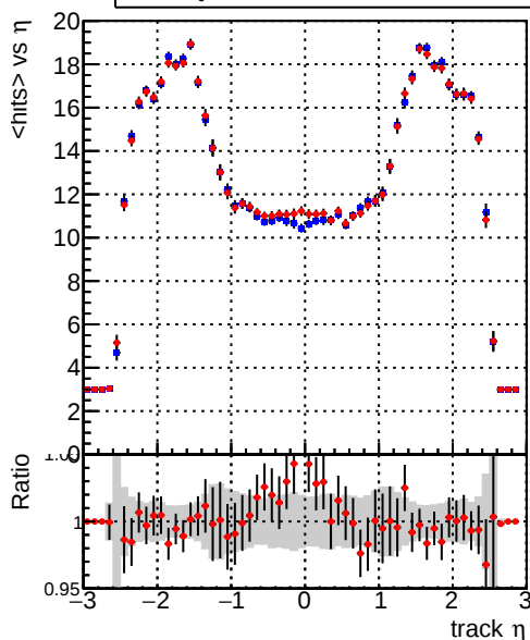
mean hits vs \eta Legend: DQM_CKF_XiMinusNOPU_base (blue line), DQM_CKF_XiMinusNOPU_retrainOldFiles125_v2_prelimWPM_epoch0 (red line)
