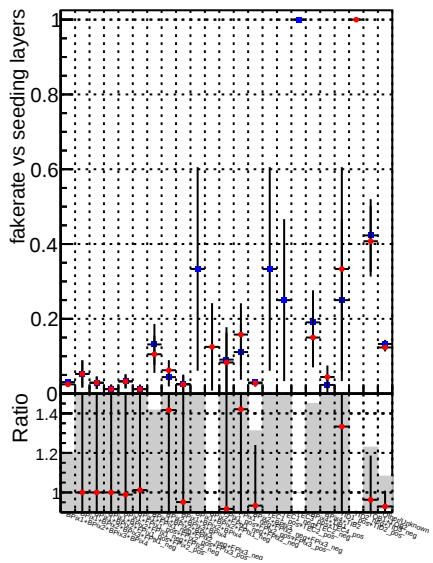
Fake rate vs. —•— DQM_CKF_XiMinusNOPU_base —•— DQM_CKF_XiMinusNOPU_retrainOldFiles125_v2_prelimWPM_epoch0
