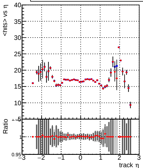
mean hits vs \eta — DQM_CKF_XiMinusNOPU_base — DQM_CKF_XiMinusNOPU_retrainOldFiles125_v2_prelimWPM_epoch0
