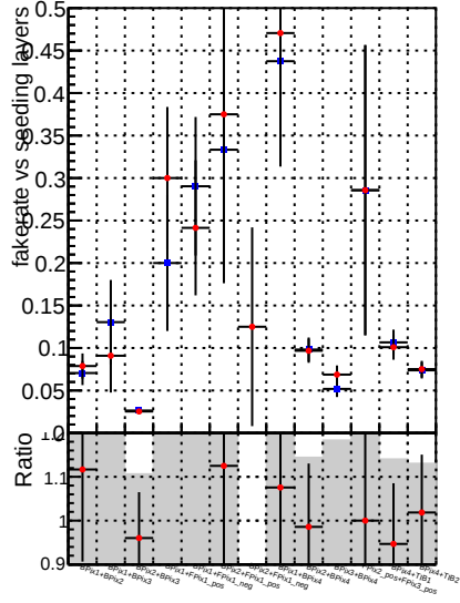
Fake rate vs. DQM_CKF_XiMinusNOPU_base DQM_CKF_XiMinusNOPU_retrainOldFiles125_v2_prelimWPM_epoch0
