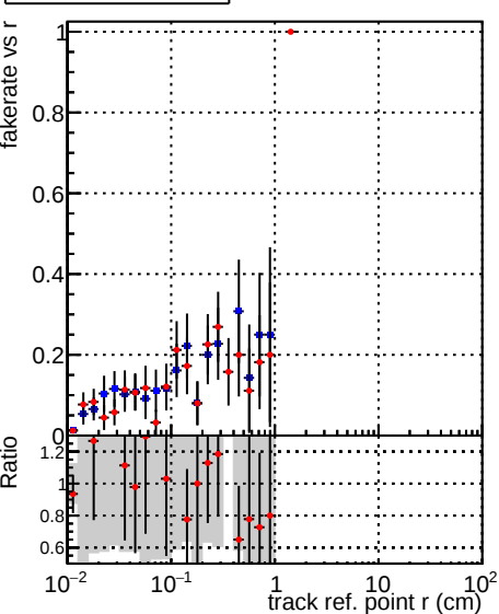
Legend: DQM_CKF_XiMinusNOPU_base (blue squares), DQM_CKF_XiMinusNOPU_retrainOldFiles125_v2_prelimWPM_epoch0 (red circles)
