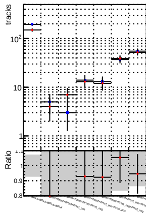
N of reco track vs. \chi^2 —●— DQM_CKF_XiMinusNOPU_base —●— DQM_CKF_XiMinusNOPU_retrainOldFiles125_v2_prelimWPM_epoch0
