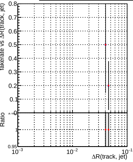
Legend: DQM_CKF_XiMinusNOPU_base (blue), DQM_CKF_XiMinusNOPU_retrainOldFiles125_v2_prelimWPM_epoch0 (red)
