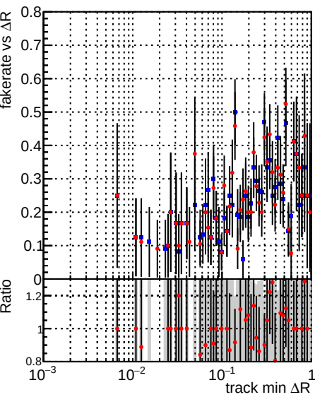
Legend: DQM_CKF_XiMinusNOPU_base (blue), DQM_CKF_XiMinusNOPU_retrainOldFiles125_v2_prelimWPM_epoch0 (red)
