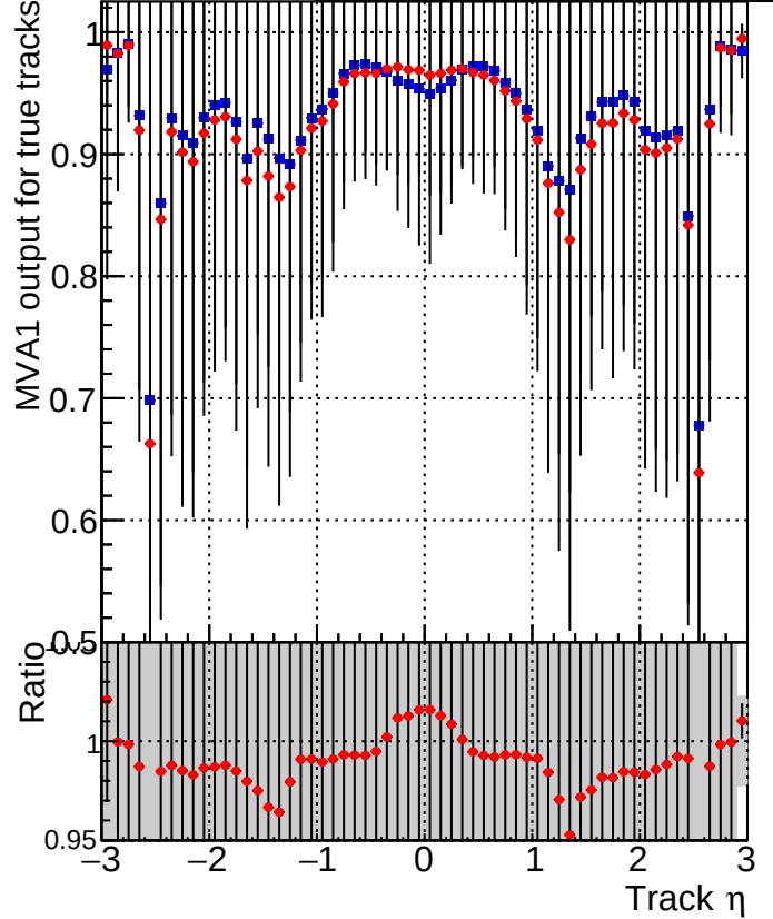
MVA1 of associated tracks (recoToSim) vs. track \eta Legend: Blue star: DQM_CKF_XiMinusNOPU_base Red diamond: DQM_CKF_XiMinusNOPU_retrainOldFiles125_v2_prelimWPM_epoch0
