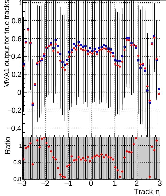
MVA1 of associated tracks (recoToSim) vs. track \eta Legend: ■ DQM_CKF_XiMinusNOPU_base ◆ DQM_CKF_XiMinusNOPU_retrainOldFiles125_v2_prelimWPM_epoch0
