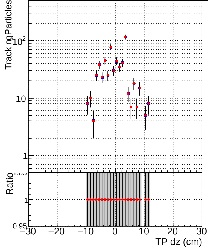
N of simulated track ■ DQM_CKF_XiMinusNOPU_base ● DQM_CKF_XiMinusNOPU_retrainOldFiles125_v2_prelimWPM_epoch0
