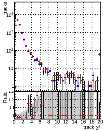
N of reco track vs. \chi^2 for DQM_CKF_XiMinusNOPU_base and DQM_CKF_XiMinusNOPU_retrainOldFiles125_v2_prelimWPM_epoch0
