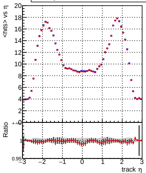
mean hit — DQM_CKF_XiMinusNOPU_base — DQM_CKF_XiMinusNOPU_retrainOldFiles125_v2_prelimWPM_epoch0
