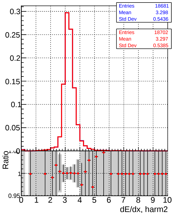
Legend: DQM_CKF_XiMinusNOPU_base (grey shaded area) DQM_CKF_XiMinusNOPU_retrainOldFiles125_v2_prelimWPM_epoch0 (red line with dots)
