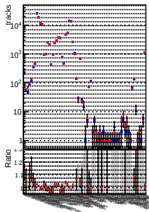
N of reco track vs. \chi^2 —•— DQM_CKF_XiMinusNOPU_base —•— DQM_CKF_XiMinusNOPU_retrainOldFiles125_v2_prelimWPM_epoch0
