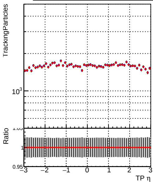
N of simulated tracks vs \eta Legend: - \blacksquare DQM_CKF_TTbase - \bullet DQM_CKF_TT_retrainOldFiles125_v2_prelimWPM_epoch4
