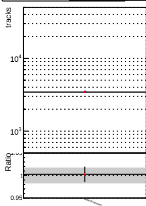
N of reco track vs. \chi^2 —●— DQM_CKF_TTbase —●— DQM_CKF_TT_retrainOldFiles125_v2_prelimWPM_epoch4
