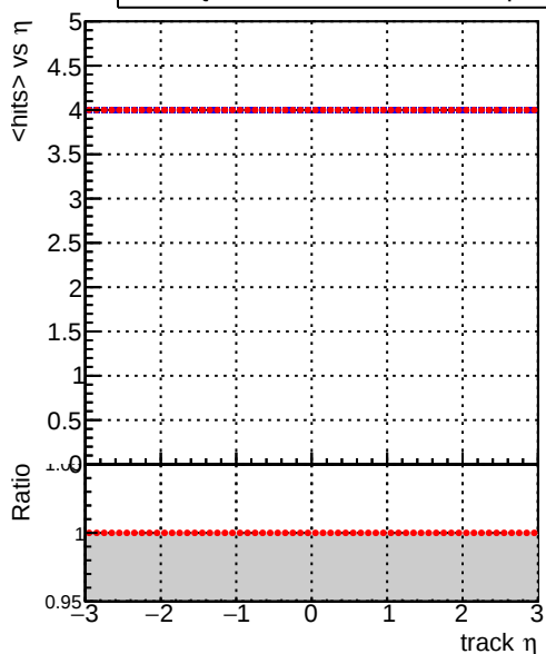
mean hits Legend: DQM_CKF_TTbase (blue line), DQM_CKF_TT_retrainOldFiles125_v2_prelimWPM_epoch4 (red line)
