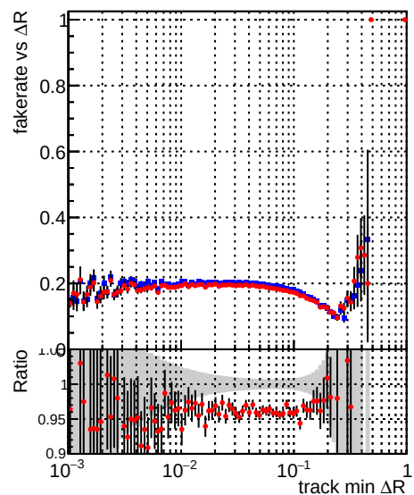
—•— DQM_CKF_TTbase —•— DQM_CKF_TT_retrainOldFiles125_v2_prelimWPM_epoch4
