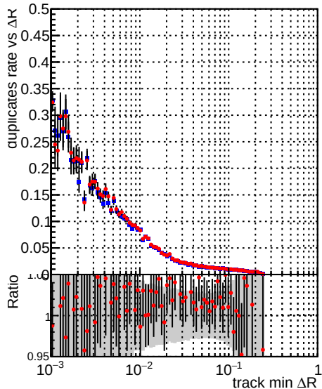
—•— DQM_CKF_TTbase —•— DQM_CKF_TT_retrainOldFiles125_v2_prelimWPM_epoch4
