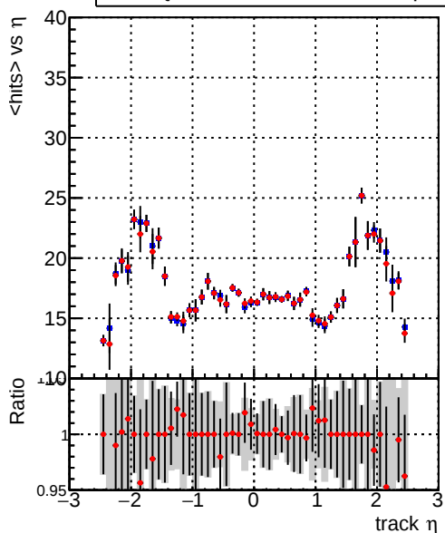
mean hits vs \eta Legend: DQM_CKF_TTbase (blue line), DQM_CKF_TT_retrainOldFiles125_v2_prelimWPM_epoch4 (red line)
