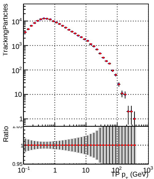
—•— DQM_CKF_TTbase —•— DQM_CKF_TT_retrainOldFiles125_v2_prelimWPM_epoch4
