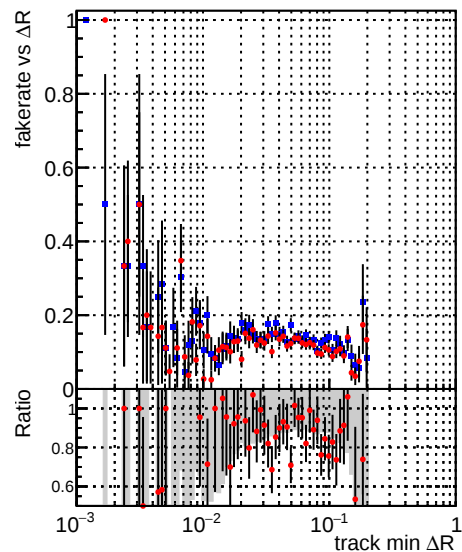
—•— DQM_CKF_TTbase —•— DQM_CKF_TT_retrainOldFiles125_v2_prelimWPM_epoch4
