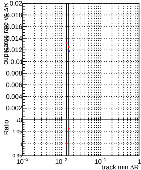
—•— DQM_CKF_TTbase —•— DQM_CKF_TT_retrainOldFiles125_v2_prelimWPM_epoch4
