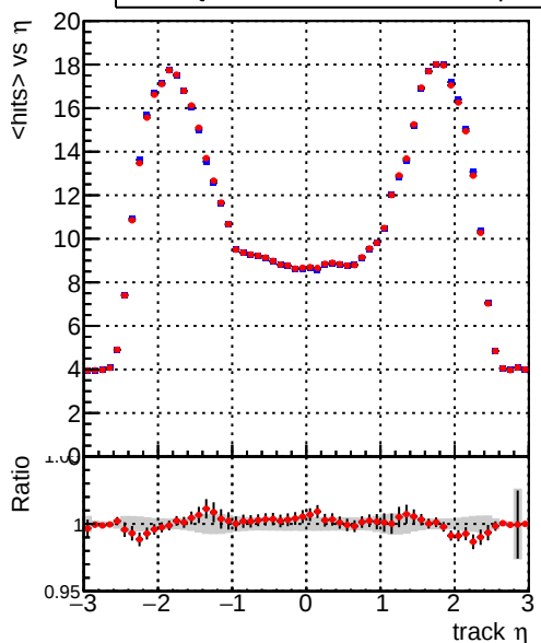
— DQM_CKF_TTbase — DQM_CKF_TT_retrainOldFiles125_v2_prelimWPM_epoch4 mean hits
