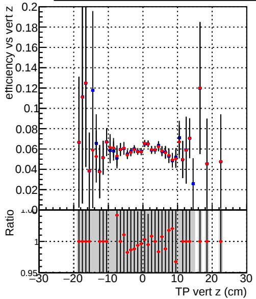
Efficiency vs. TP vert z (cm) Legend: —●— DQM_CKF_TTbase, —●— DQM_CKF_TT_retrainOldFiles125_v2_prelimWPM_epoch4
