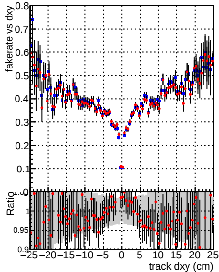
—●— DQM_CKF_TTbase —●— DQM_CKF_TT_retrainOldFiles125_v2_prelimWPM_epoch4
