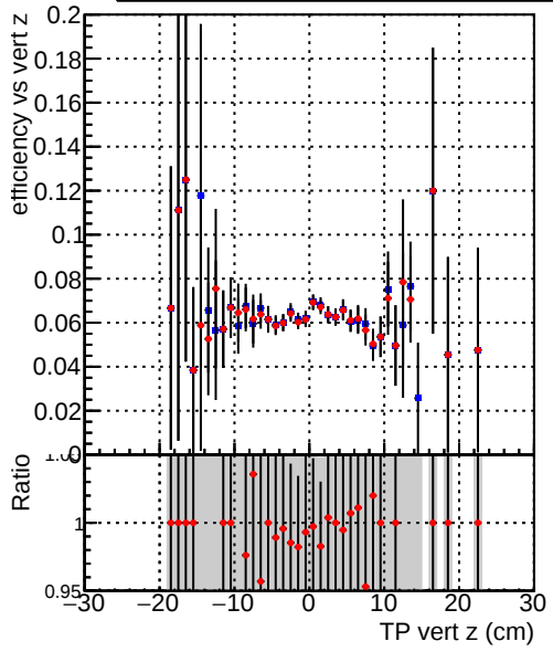
Efficiency vs. TP vert z — DQM_CKF_TTbase — DQM_CKF_TT_retrainOldFiles125_v2_prelimWPM_epoch4
