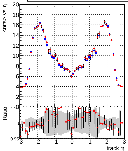
mean hits vs \eta Legend: DQM_CKF_TTbase (blue line), DQM_CKF_TT_retrainOldFiles125_v2_prelimWPM_epoch4 (red line)
