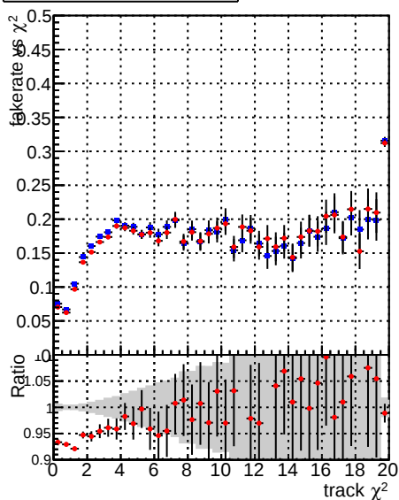
Fake rate vs. —●— DQM_CKF_TTbase —●— DQM_CKF_TT_retrainOldFiles125_v2_prelimWPM_epoch4
