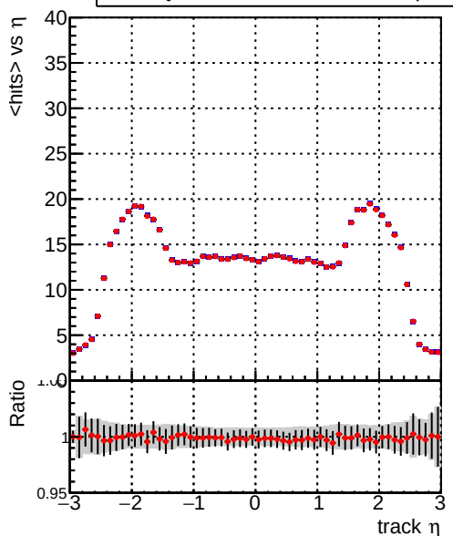
mean hits — DQM_CKF_TTbase — DQM_CKF_TT_retrainOldFiles125_v2_prelimWPM_epoch4
