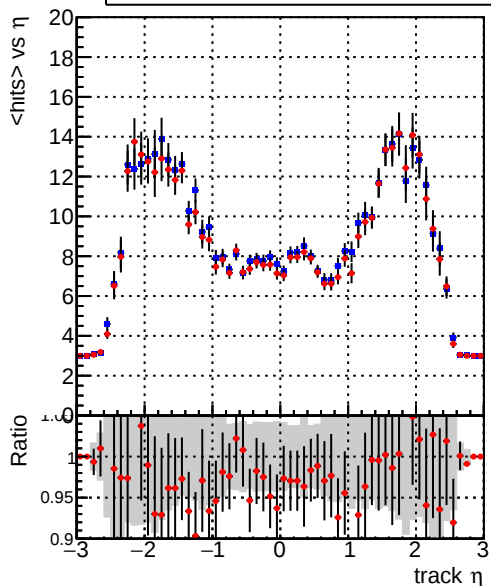
— DQM_CKF_TTbase — DQM_CKF_TT_retrainOldFiles125_v2_prelimWPM_epoch4 mean hits
