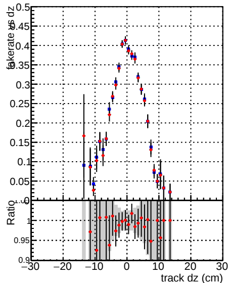
Fake rate vs dz DQM_CKF_TTbase (blue dots) DQM_CKF_TT_retrainOldFiles125_v2_prelimWPM_epoch4 (red dots)
