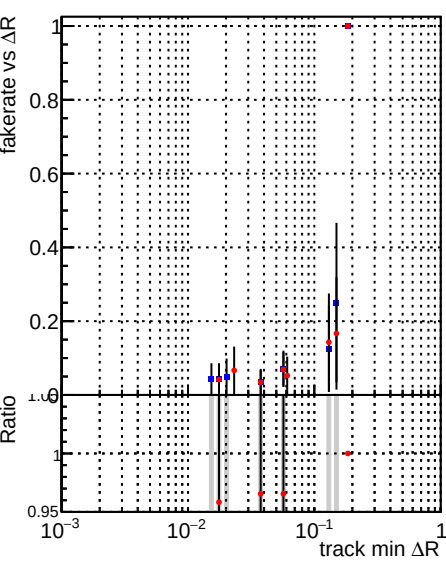
Legend: DQM_CKF_TTbase (blue squares), DQM_CKF_TT_retrainOldFiles125_v2_prelimWPM_epoch4 (red circles)
