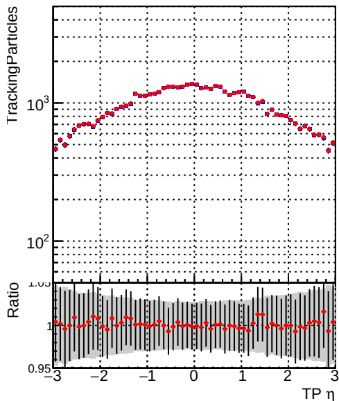
—•— DQM_CKF_TTbase —•— DQM_CKF_TT_retrainOldFiles125_v2_prelimWPM_epoch4
