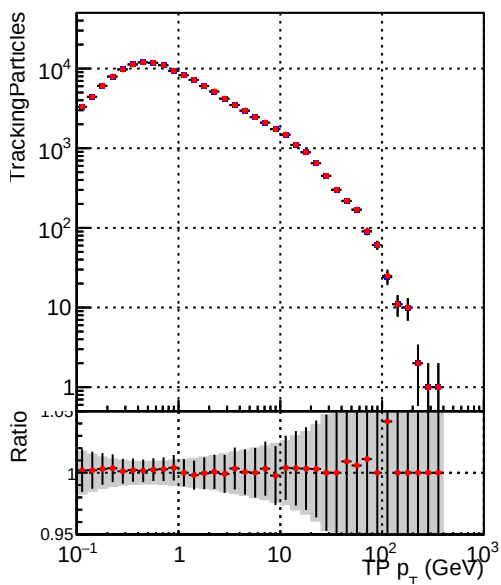
—•— DQM_CKF_TTbase —•— DQM_CKF_TT_retrainOldFiles125_v2_prelimWPM_epoch4
