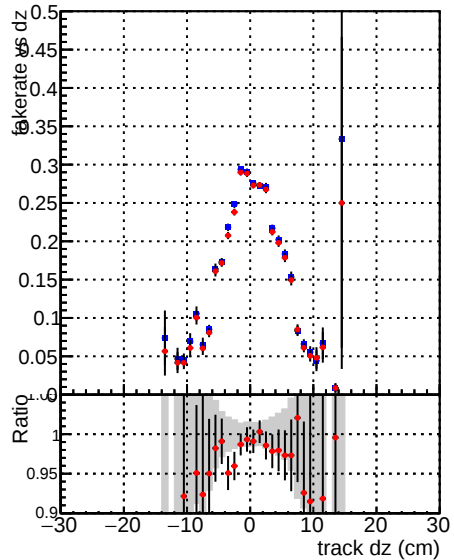
—●— DQM_CKF_TTbase —●— DQM_CKF_TT_retrainOldFiles125_v2_prelimWPM_epoch4
